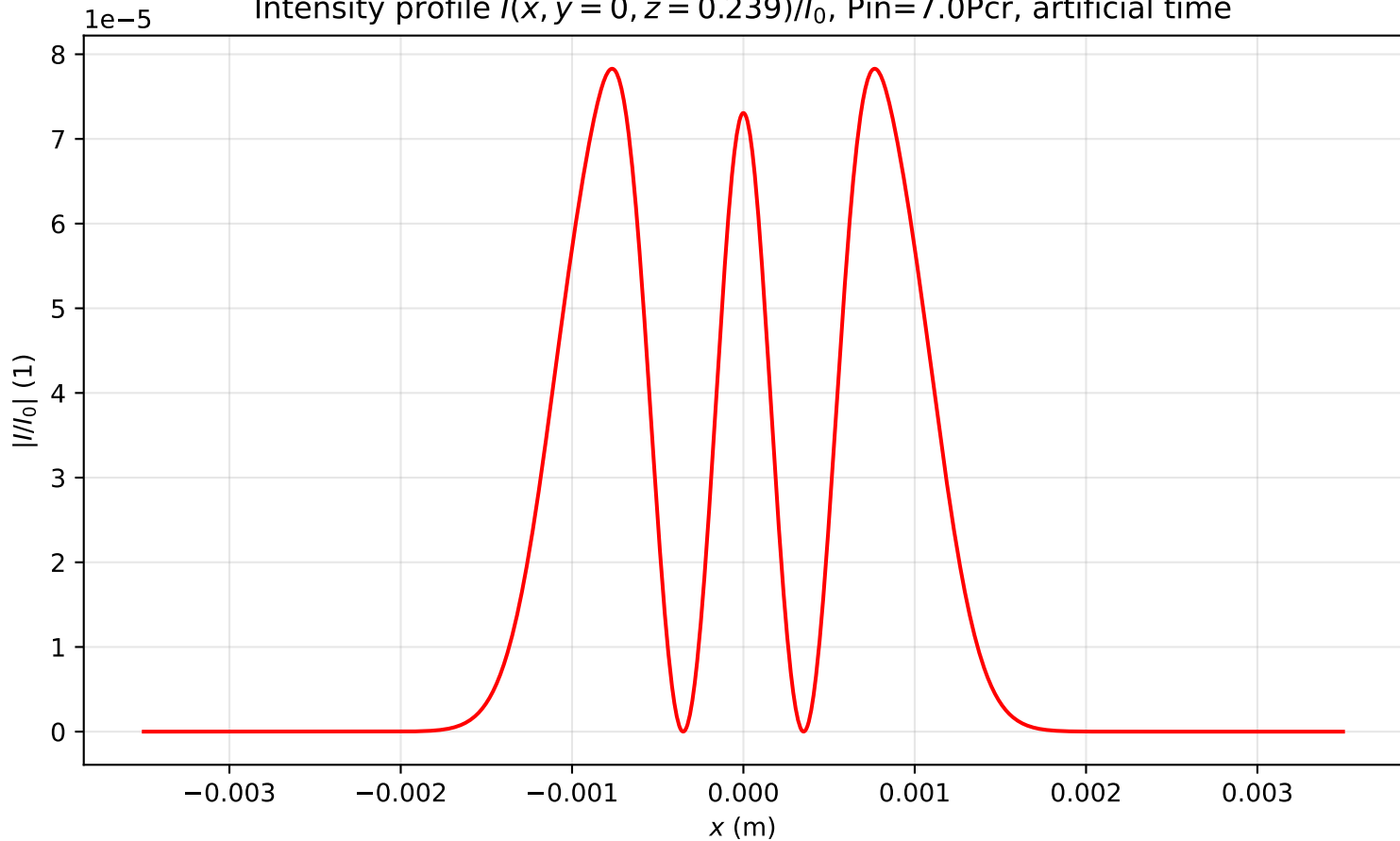
Intensity profile I(x, y = 0, z = 0.239)/I_0 , P_{in}=7.0P_{cr} , artificial time
